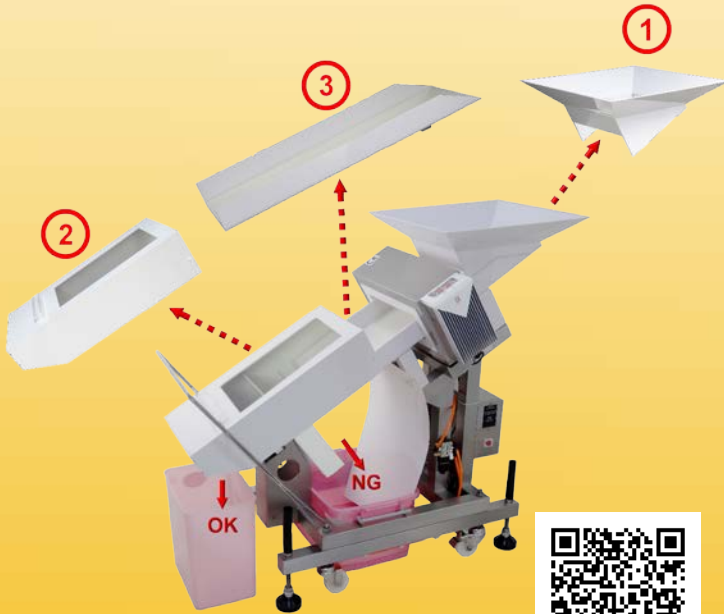
MD3010 Slide-Down Channel
